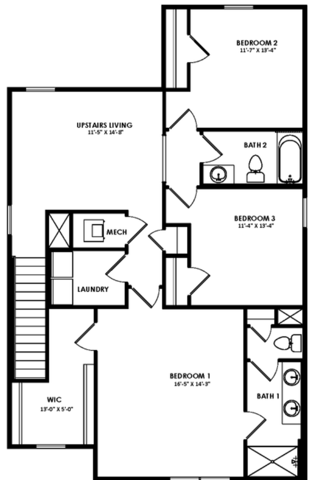
Second Floor
