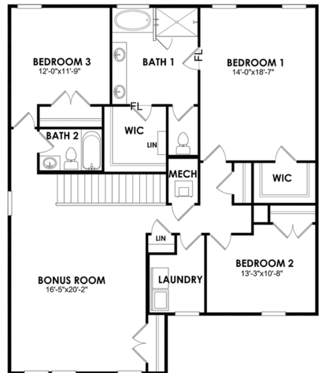
Second Floor - Elevation JS & KS
