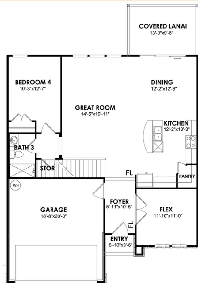
First Floor - Elevation JS
