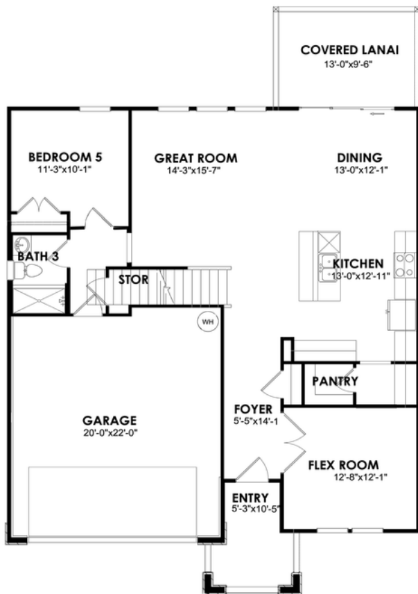
First Floor - Elevation JS
